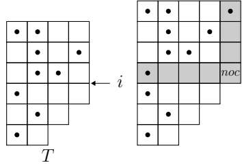
(a) Bijection between NOC_{a,b}(\mathcal{T}_n) and pairs (T, i) .
