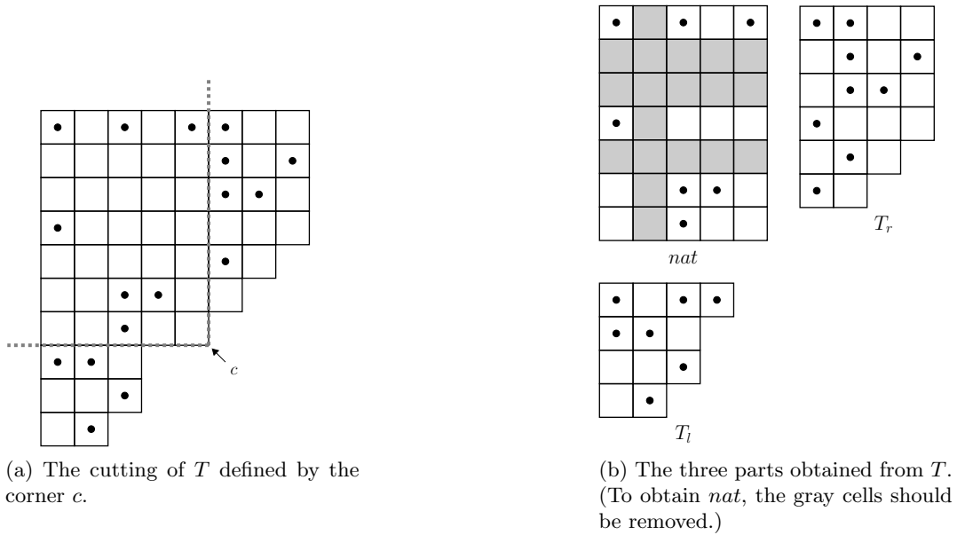
Figure 9: An example of the bijection of Lemma 4.6.
