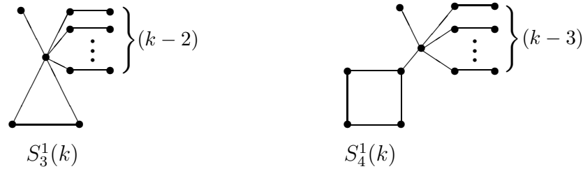
Figure 1. The graphs S_3^1(k) and S_4^1(k)
