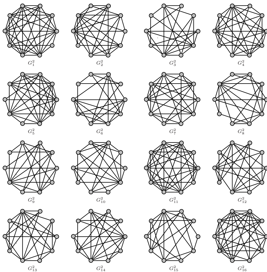
Figure 2.2: The 25 quadratic borderenergetic graphs of order 10 ( G_1^2 – G_{16}^2 )
