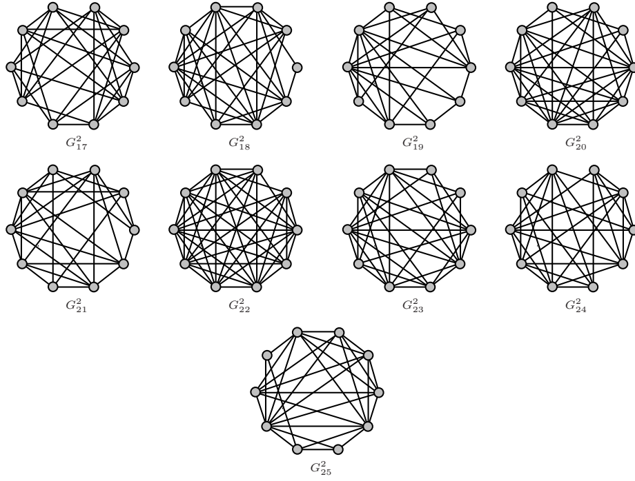
Figure 2.3: The 25 quadratic borderenergetic graphs of order 10 ( G^2_{17} – G^2_{25} )
