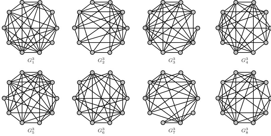
Figure 2.4: The 8 cubic borderenergetic graphs of order 10
