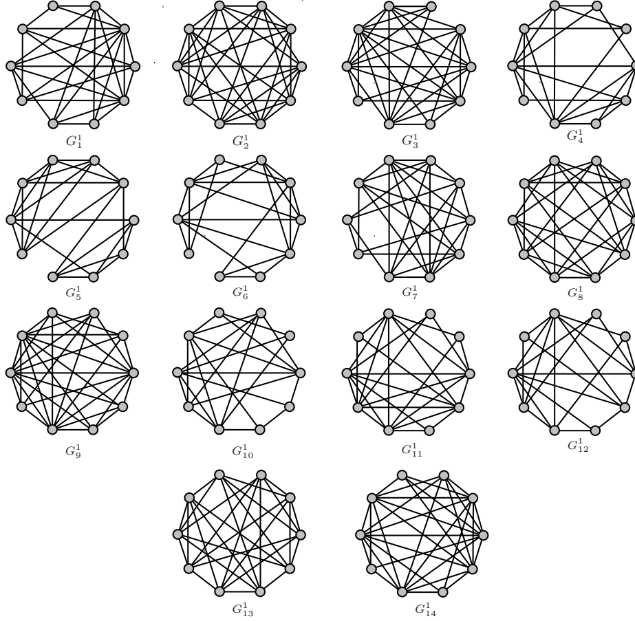
Figure 2.1: The 14 integral borderenergetic graphs of order 10
